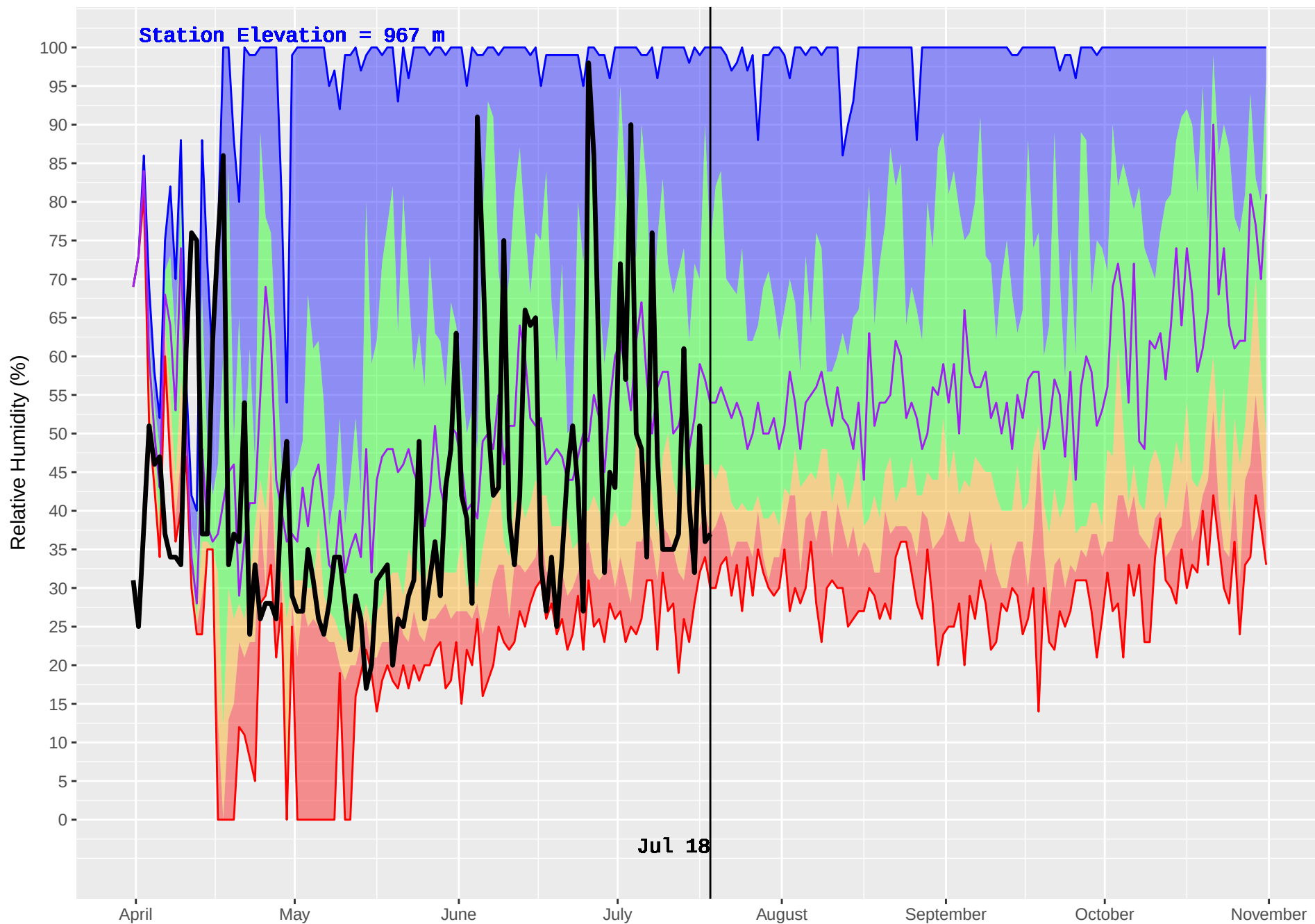
WONOWON (136) : Historical (1990–2016) and Current (2018) Daily Relative Humidity
