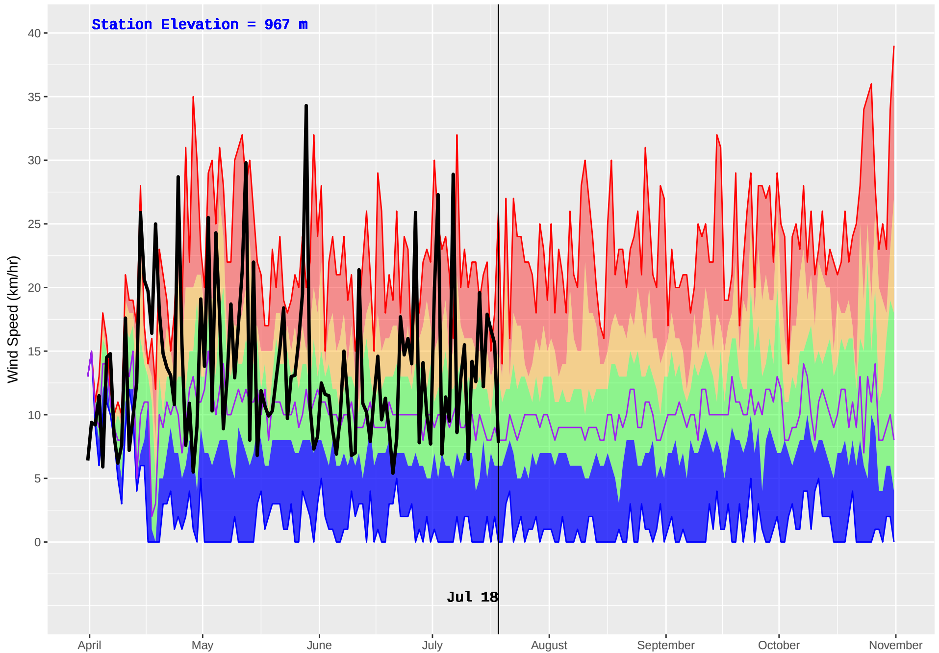
WONOWON (136) : Historical (1990–2016) and Current (2018) Daily Wind Speed
