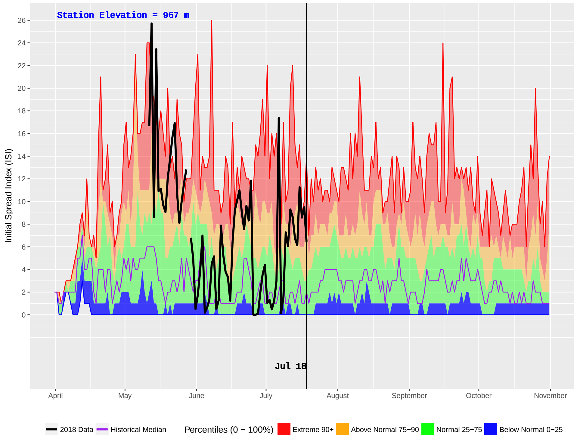
WONOWON (136) : Historical (1990–2016) and Current (2018) Daily Initial Spread Index (ISI)
