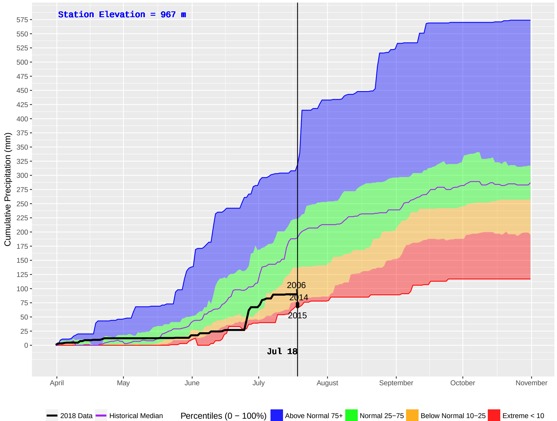
WONOWON (136) : Historical (1990–2016) and Current (2018) Daily Cumulative Precipitation
