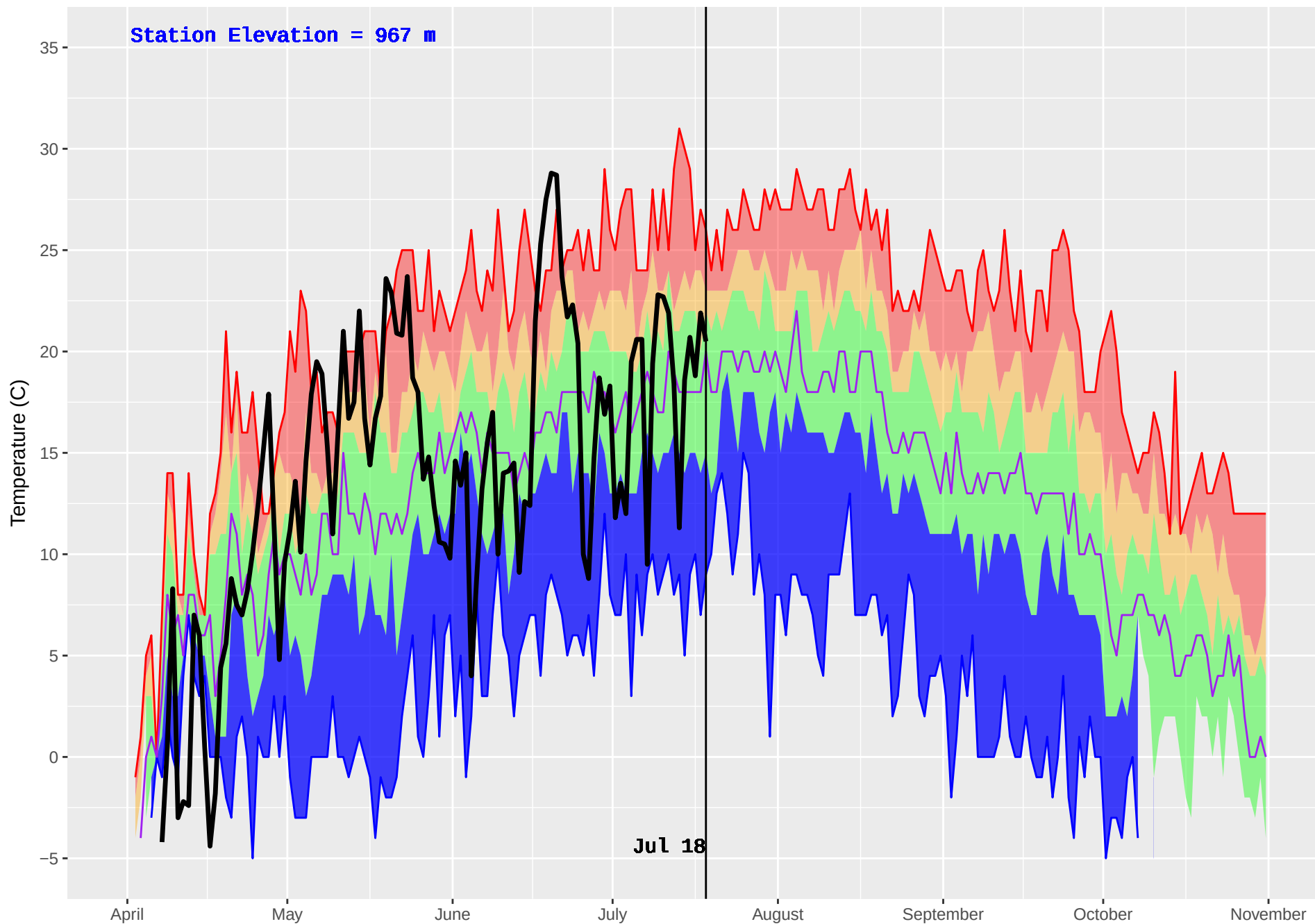
WONOWON (136) : Historical (1990–2016) and Current (2018) Daily Temperature
