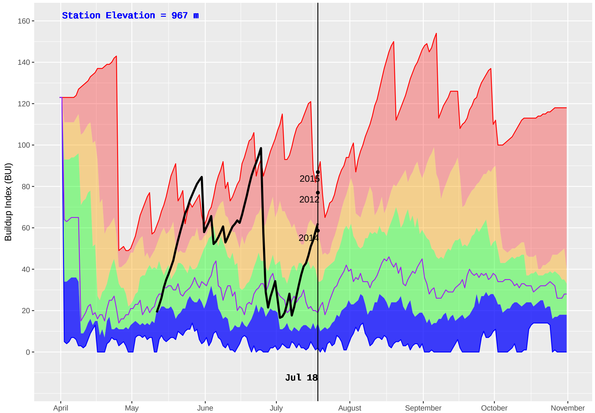
WONOWON (136) : Historical (1990–2016) and Current (2018) Daily Buildup Index (BUI)
