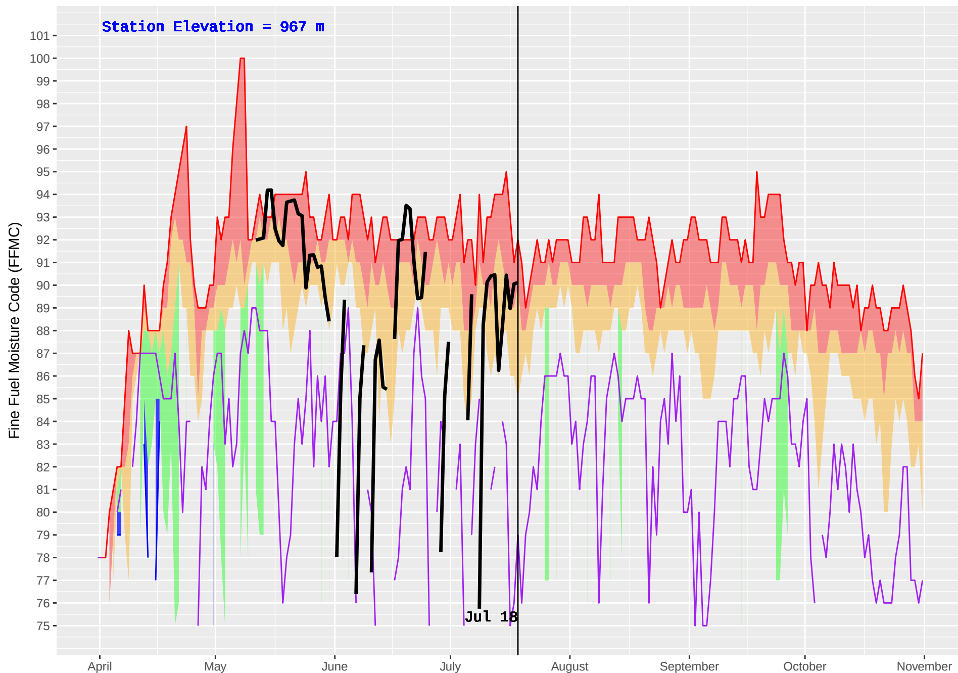
WONOWON (136) : Historical (1990–2016) and Current (2018) Daily Fine Fuel Moisture Code (FFMC)
